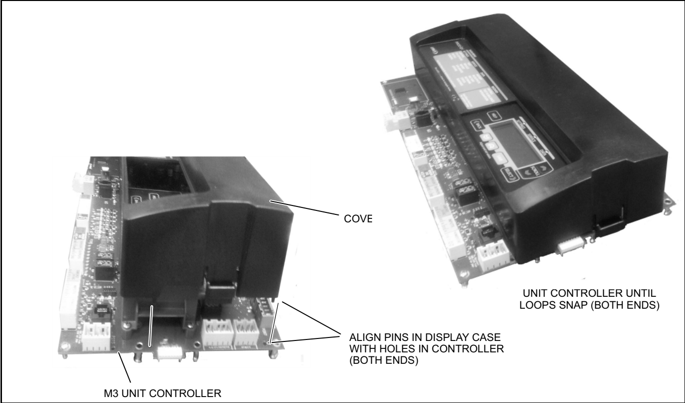
Figure 2. Installing M3 Unit Controller Cover
