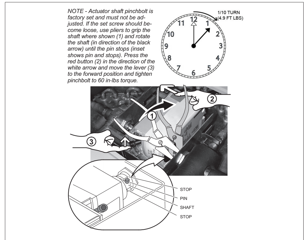
Figure 18. Re-Aligning Pinch Bolt
