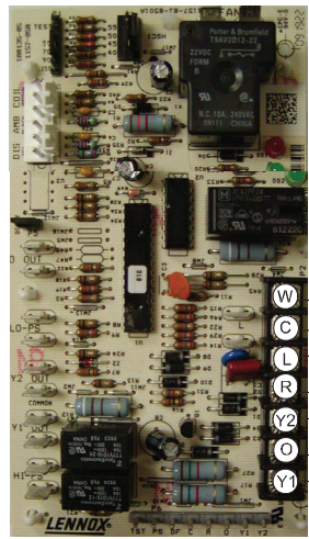
OUTDOOR UNIT DEFROST BOARD (HP)
