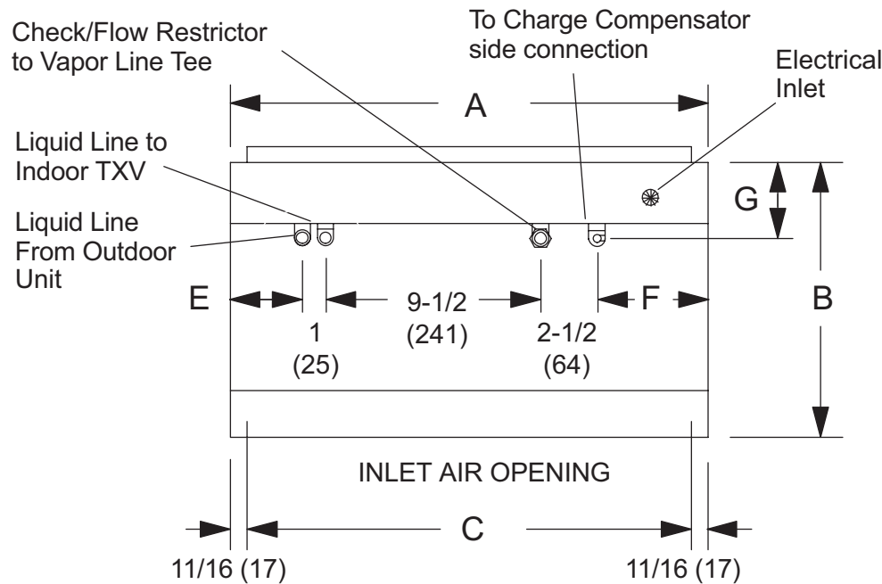
Figure 2. Unit Dimensions
