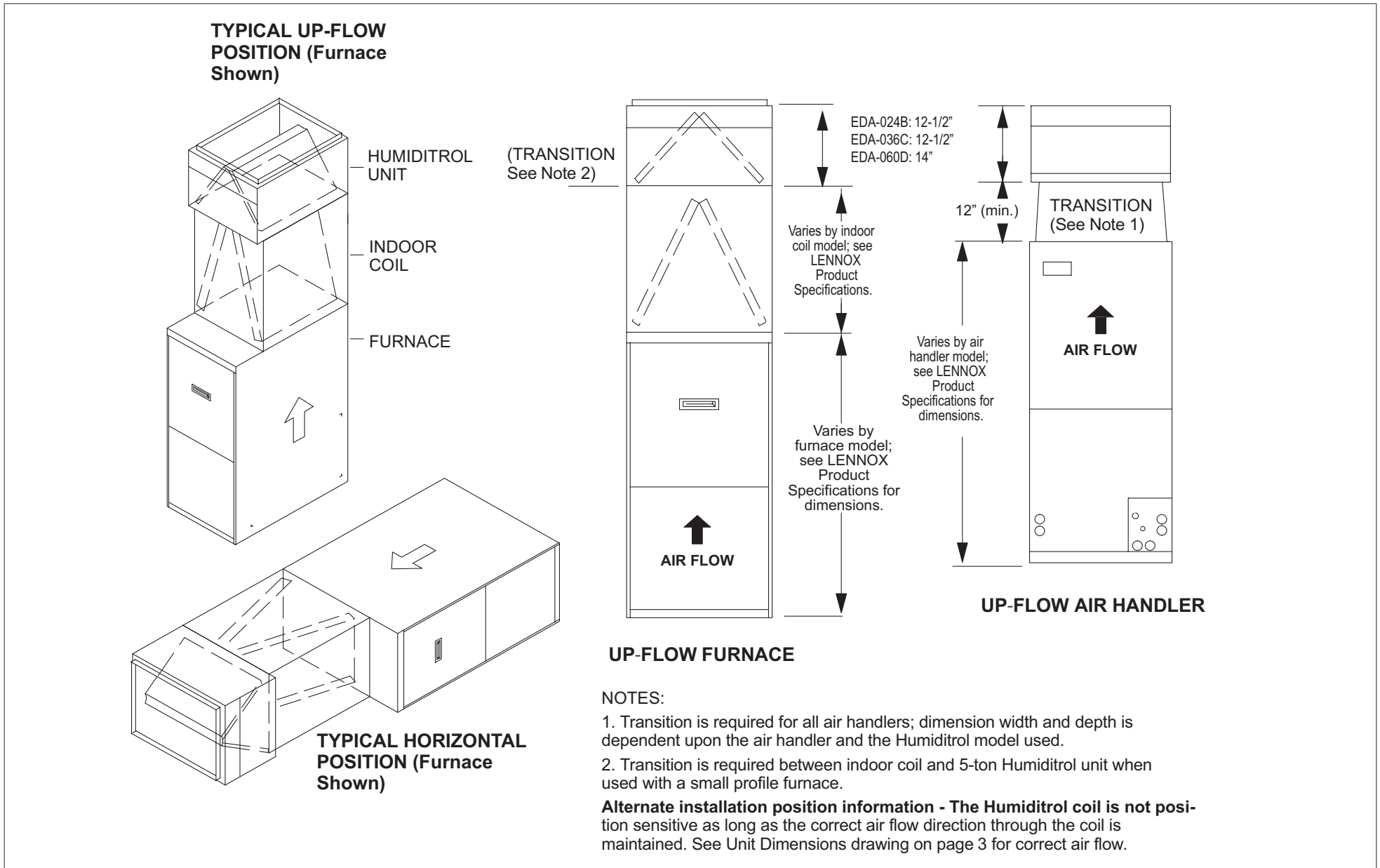
Figure 3. Installation Arrangements (Horizontal and Up-flow)
