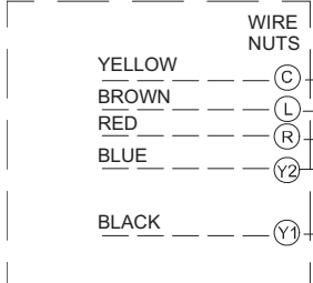
OUTDOOR UNIT CONTROL WIRES (AC)
