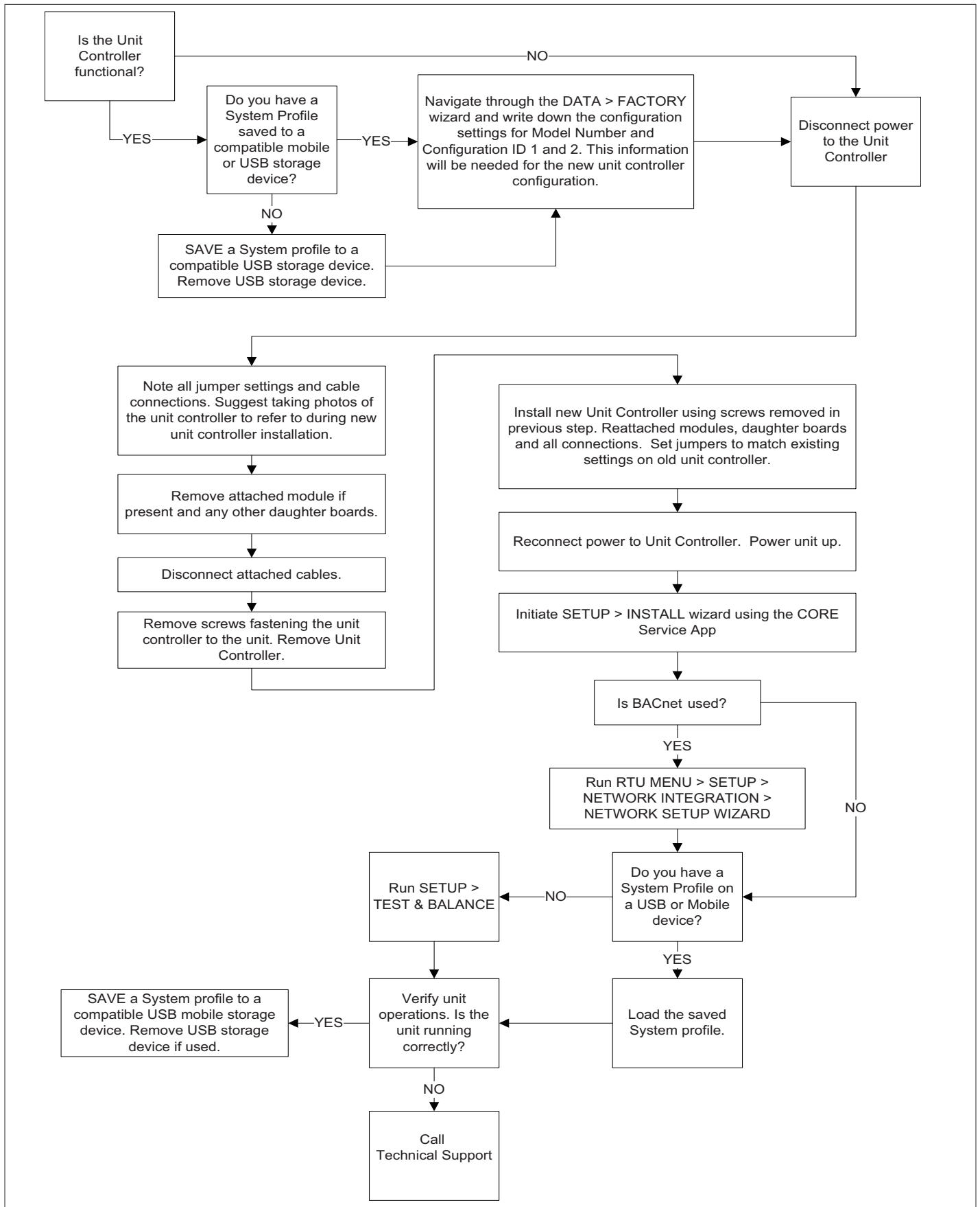
Figure 1. Unit Controller Replacement
