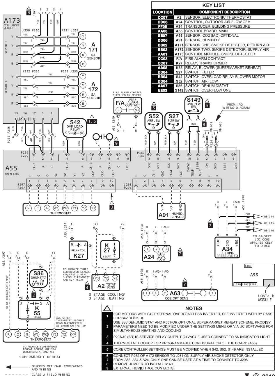
WIRING DIAGRAM FLOW
